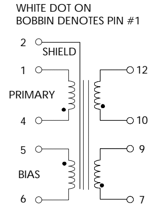
FIGURE 1: SCHEMATIC DIAGRAM
